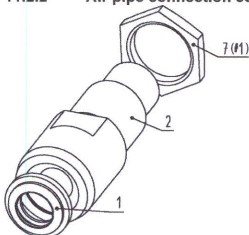
Fig. 36 Air pipe connection 330.277.04 "10.05"
