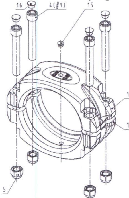
Fig. 160 Muff coupling 010.614.36 "10.04"
