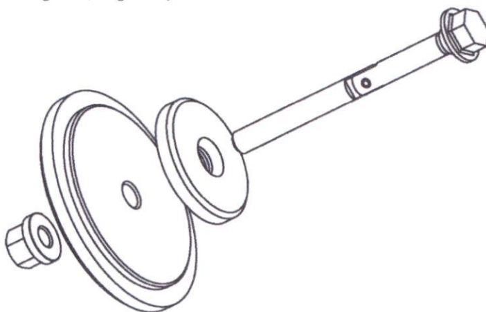
Fig. 170 Mounting device for bushes in support
