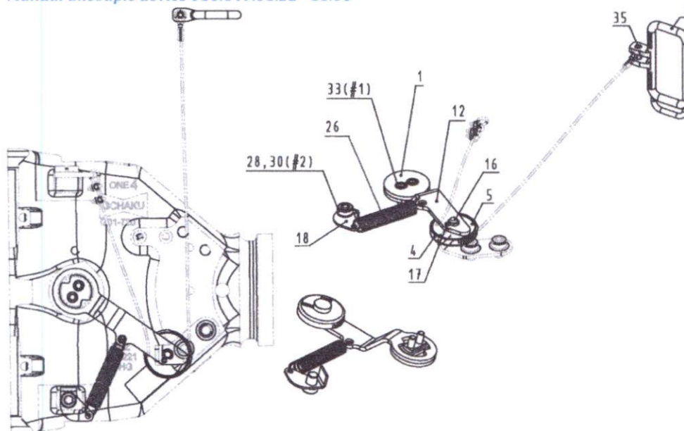
Fig. 140 Manual uncouple device 010.649.01.22 "11.00"
