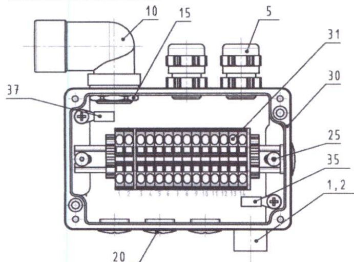
Fig. 158 Terminal box 010.775.18.01
