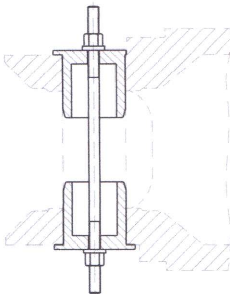
Fig. 165 Mounting device for METALOPLAST bushes
