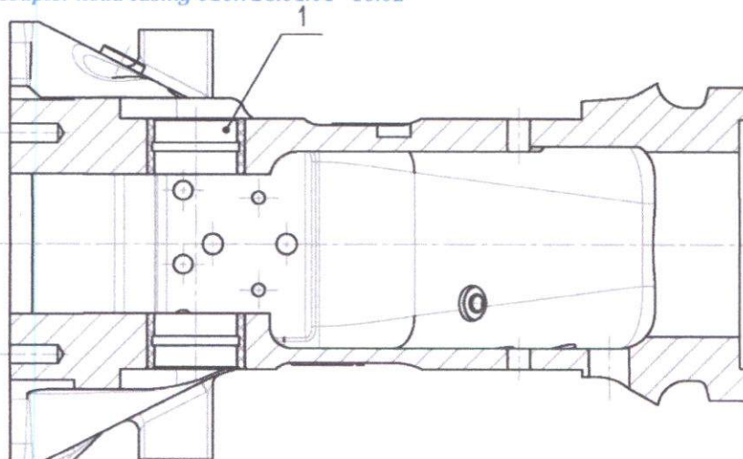
Fig. 136 Coupler head casing 010.726.01.01 "10.02"
