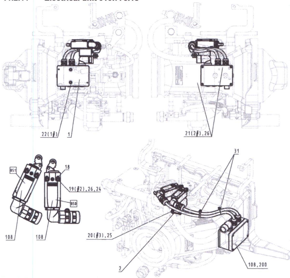
Fig. 156 Electrical unit 010.775.18
