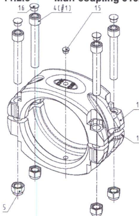
Fig. 40 Muff coupling 010.614.36 "10.04"
