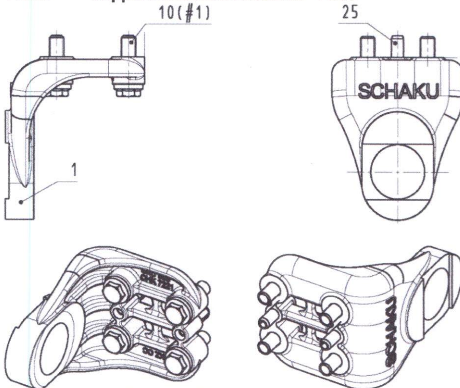
Fig. 38 Support bracket 010.652.14 "11.00"
