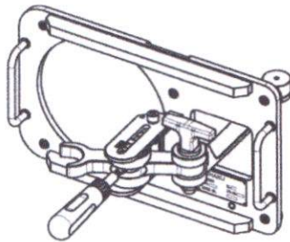
Fig. 162 Coupler lock backlash gauge
