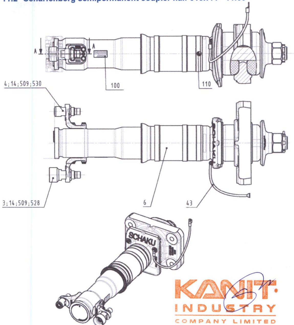
Fig. 34 Scharfenberg semipermanent coupler half 010.777 "11.00"
