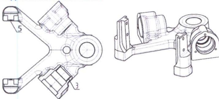
Fig. 152 Support bracket 010.718.10.01
