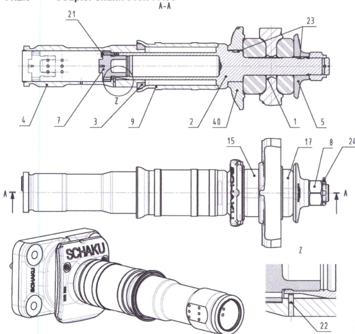
Fig. 37 Coupler shank 010.777.06
