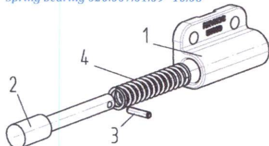
Fig. 139 Spring bearing 020.007.01.09 "10.08"
