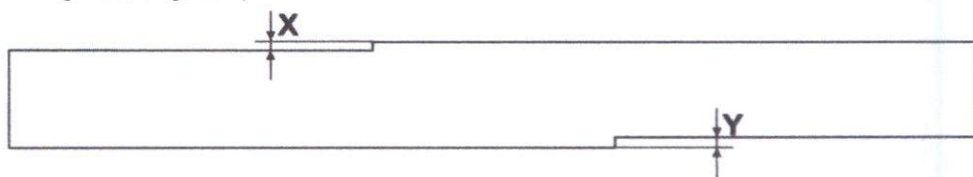
Fig. 166 Gauge for measuring the projection of the electric head
