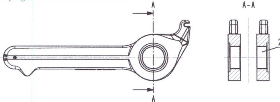
Fig. 137 Coupling link with bushes 010.164.01.08 "10.04"
