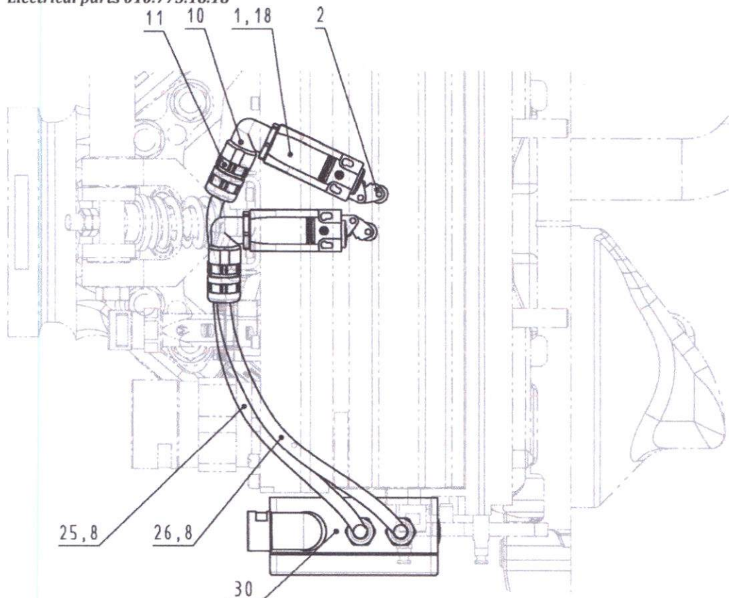
Fig. 157 Electrical parts 010.775.18.18
