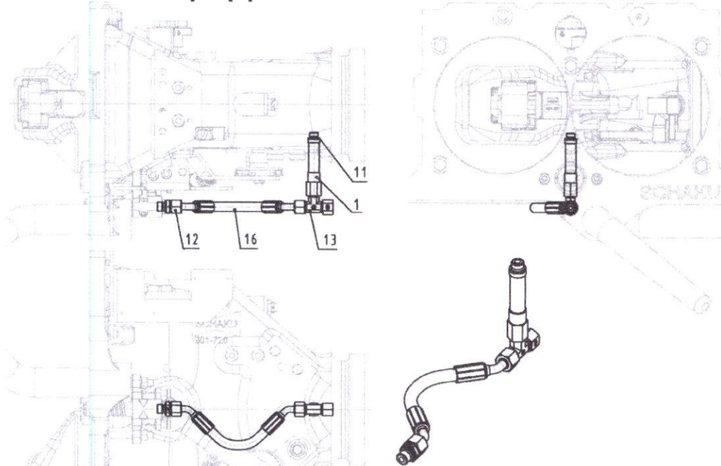
Fig. 154 Uncouple pipe 010.700.12 "10.01"
