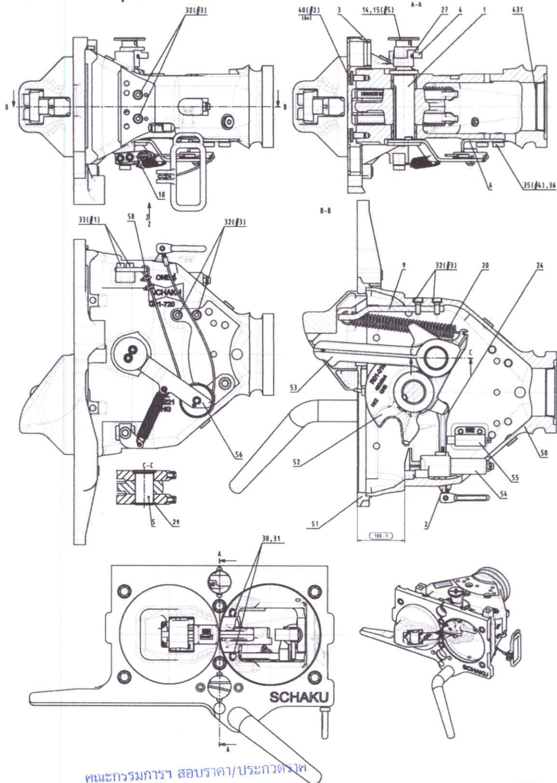
Fig. 135 Coupler head 010.752.01
