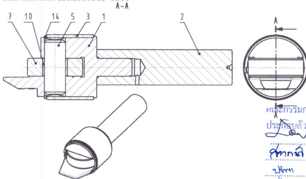
Fig. 151 Stem with roller 330.500.10.02 "10.01"
