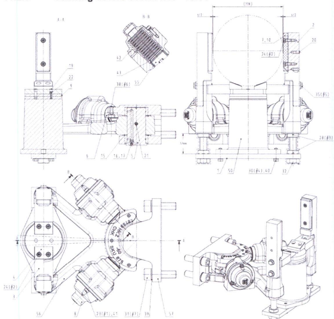
Fig. 150 Centring device 330.511.10 "10.04"
