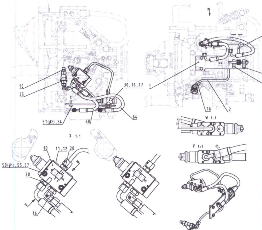
Fig. 155 Pneumatic unit 010.775.15 "10.01"
