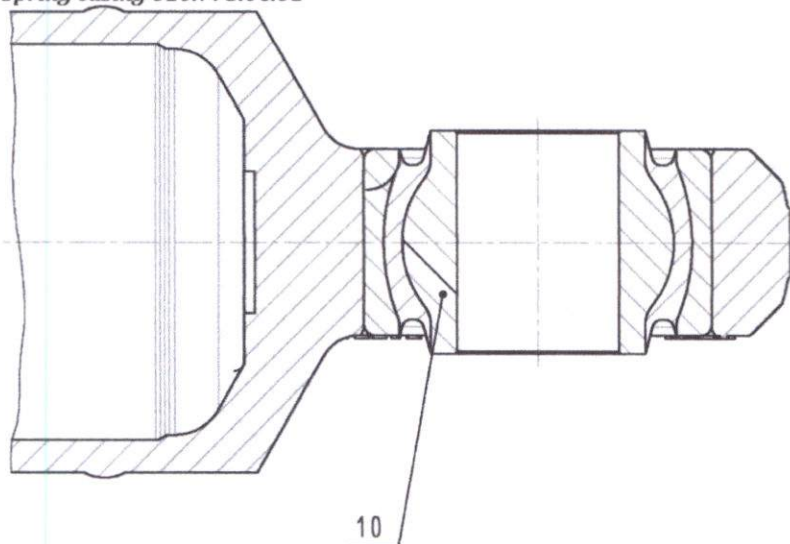
Fig. 146 Spring casing 010.775.06.01
