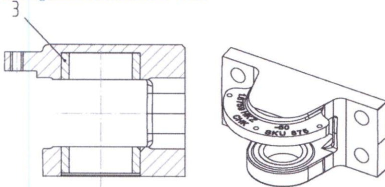
Fig. 153 Bearing bracket 010.613.10.01 "10.01"
