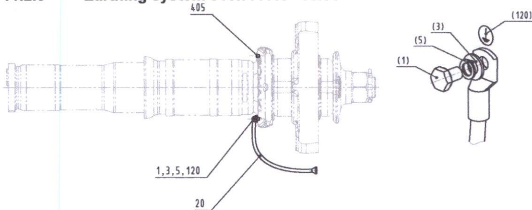
Fig. 39 Earthing system 010.777.43 "10.01"
