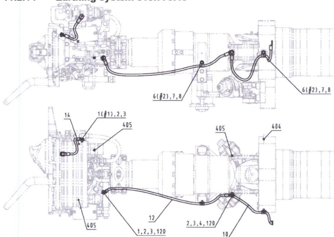
Fig. 161 Earthing system 010.775.43
