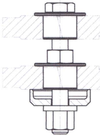
Fig. 163 Mounting device for gluing bushes into coupling link
