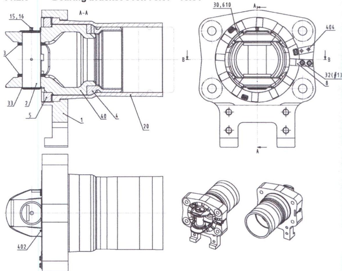
Fig. 147 Bearing bracket 010.775.07 "10.01"
