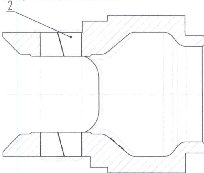
Fig. 148 Bearing bracket 050.117.07.01 "10.02"
